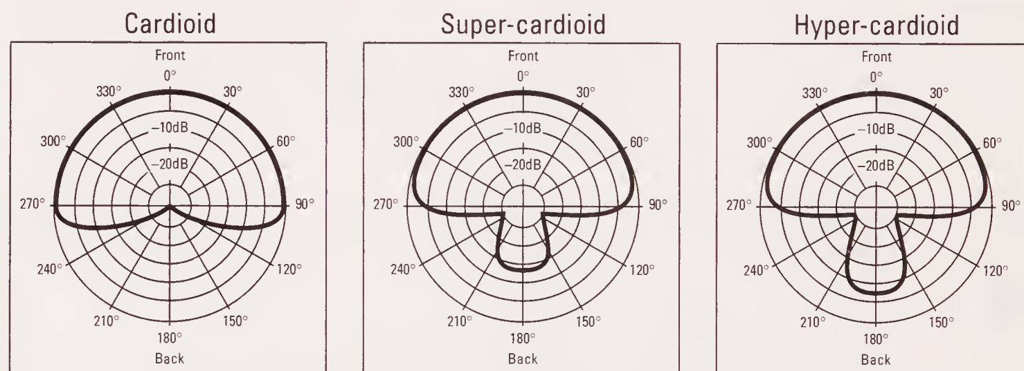
Figure 2-2: Various cardioid patterns of different condenser micro- phones.
