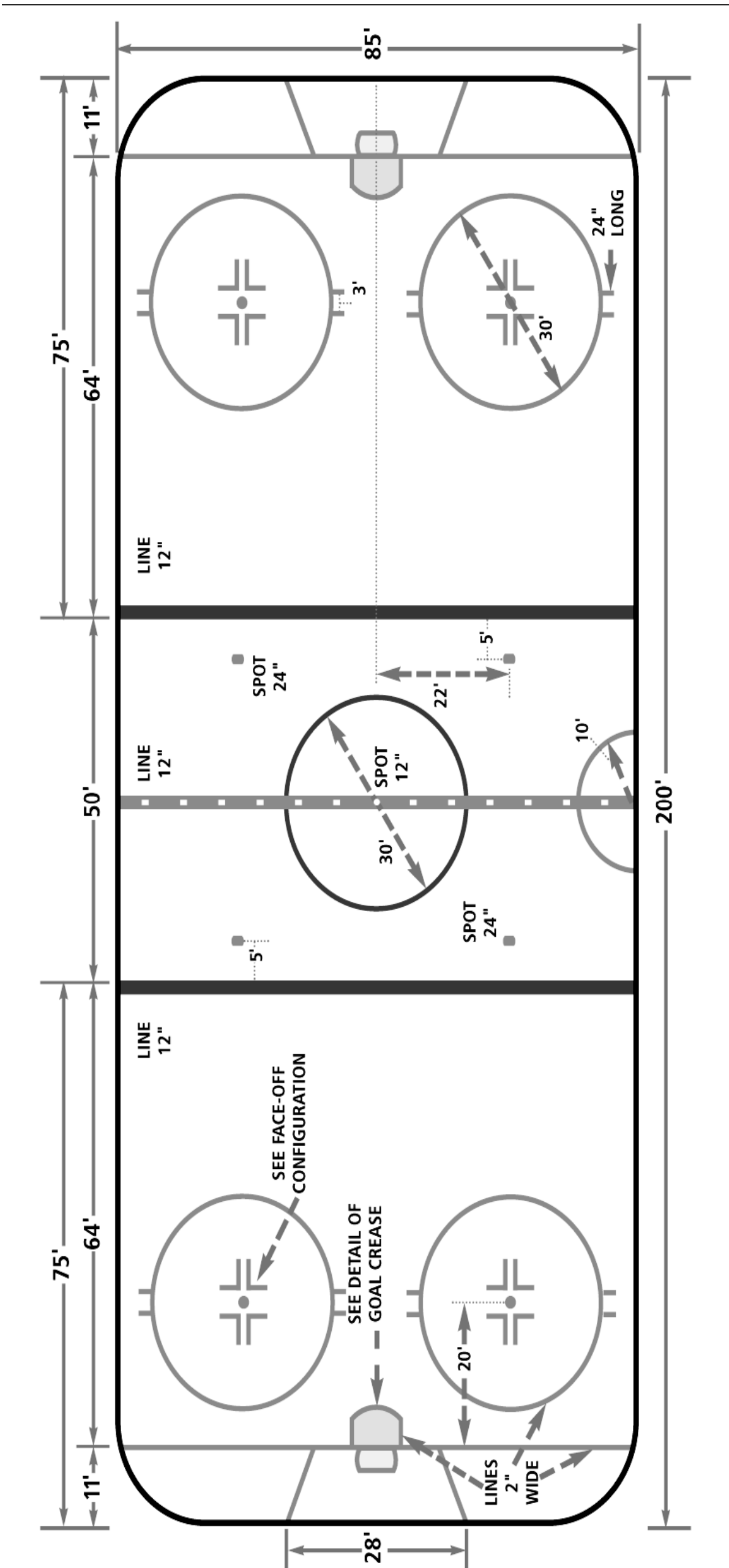
OFFICIAL DIMENSIONS OF RINK SURFACE
